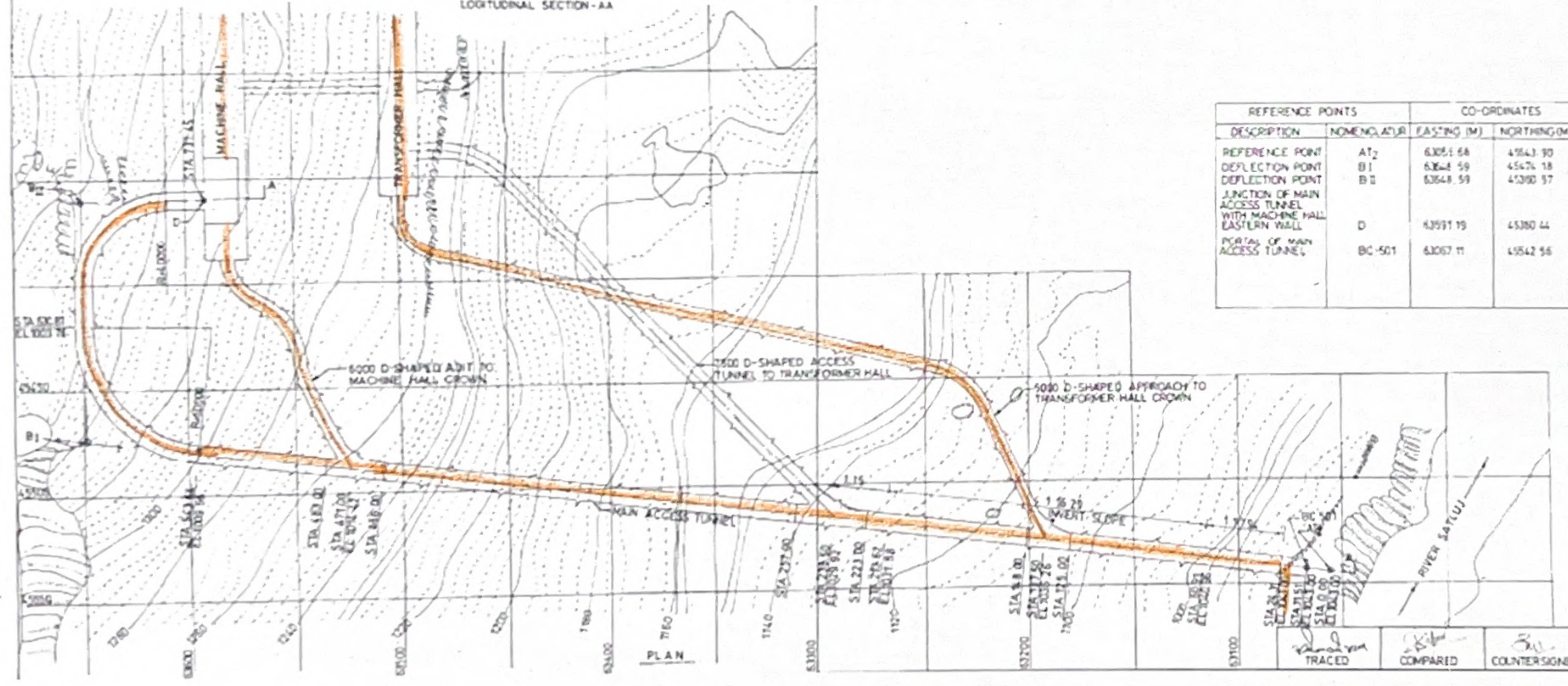
PLAN :- SHOWING PAINTING WORK ON VENTILATION DUCTS IN POWER-HOUSE CMAT, CROWN OF MACHINE HALL AND CROWN OF TRANSFORMER HALL
