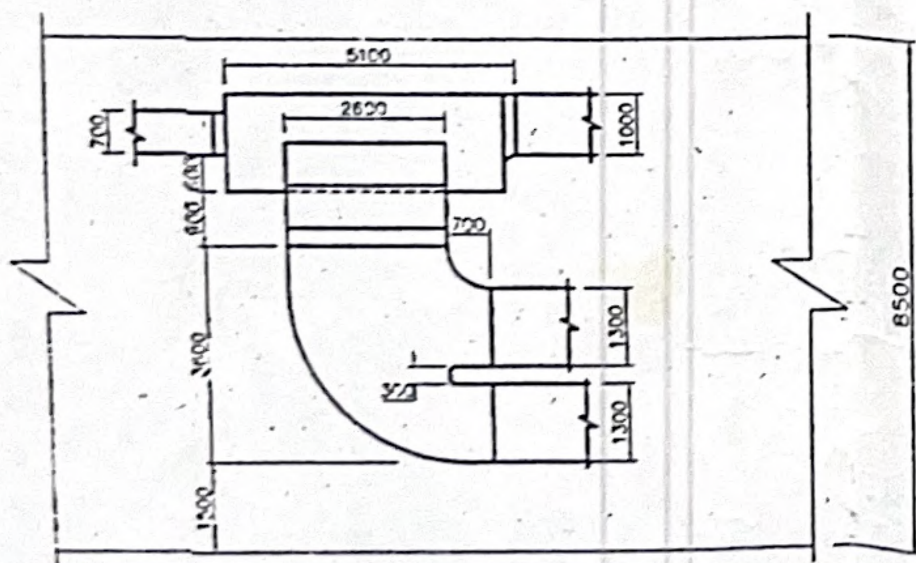
DETAIL OF DUCT AT VIEW-D
